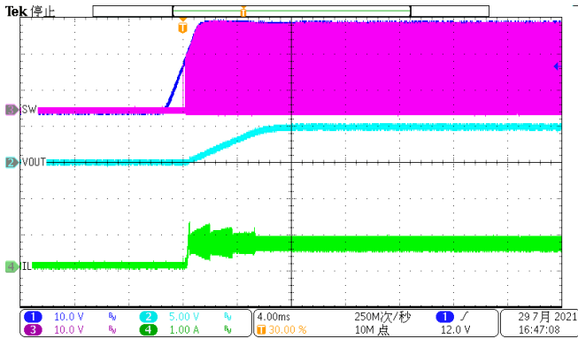
Figure 11. Power up(Iload=0.6A)
