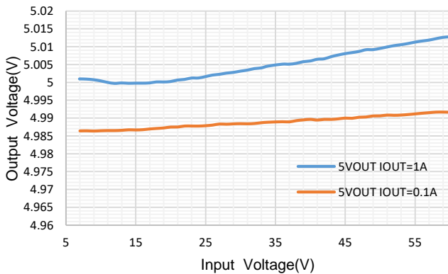
Figure 6. Line Regulation
