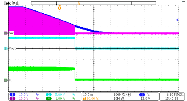
Figure 12. Power down(Iload=1A)
